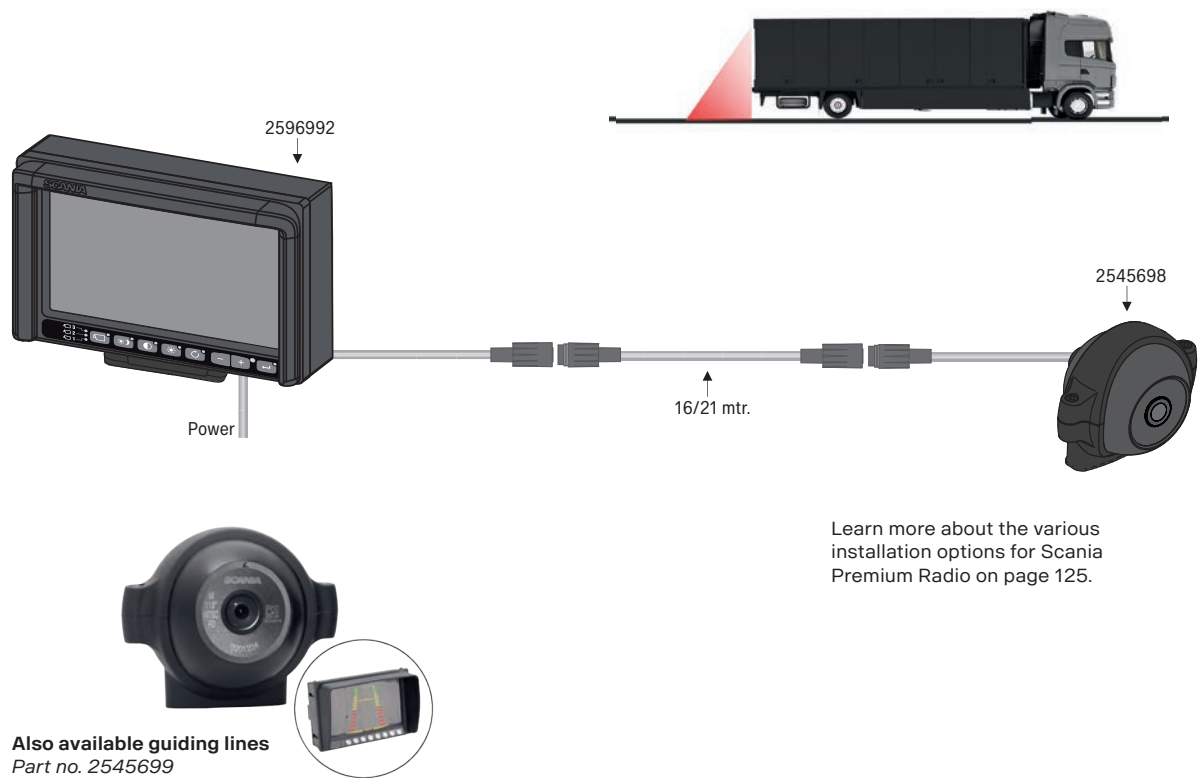
Famos rear view (rigid truck) configuration drawing
