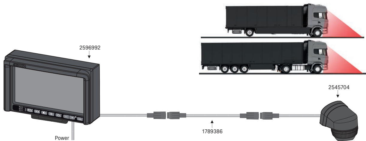
Front view configuration drawing
