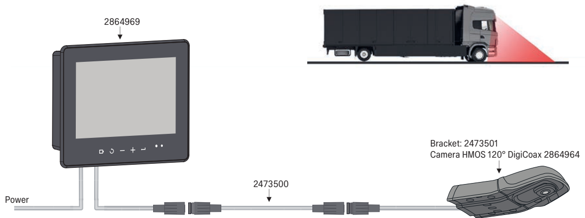
Front view HD configuration drawing
