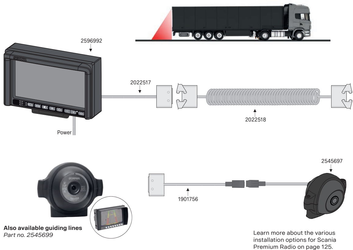
Famos rear view (trailer trucks) configuration drawing
