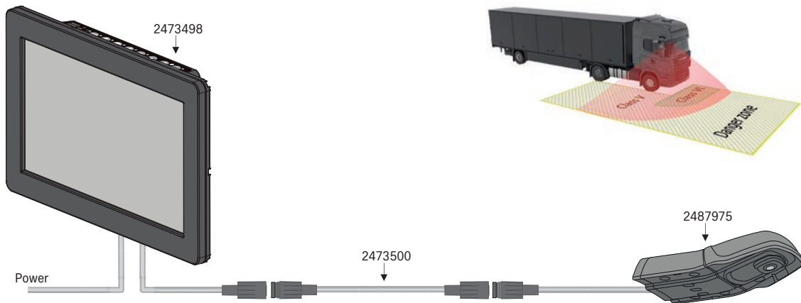
CornerEye configuration drawing
