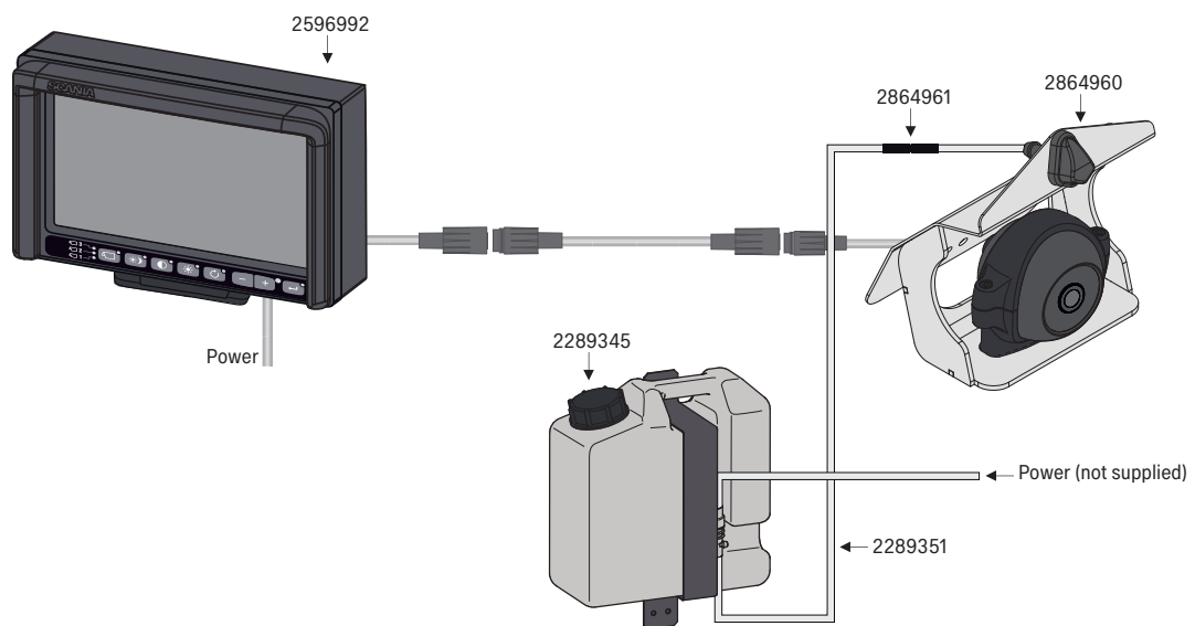
Nozzle lens cleaner configuration drawing
